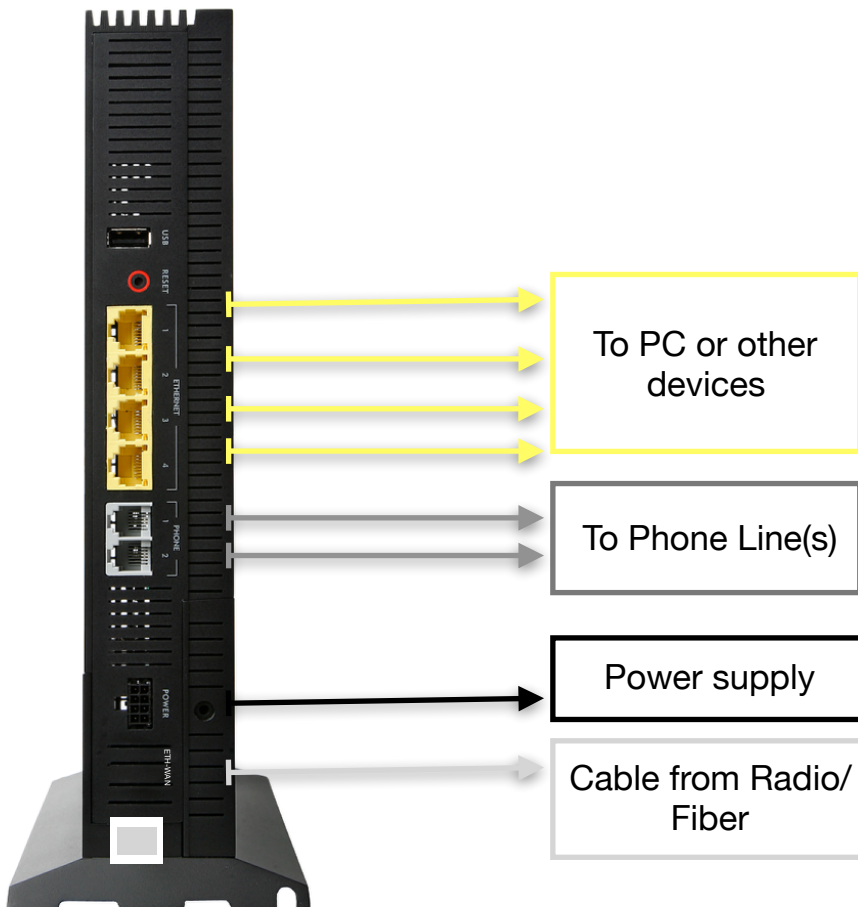
Back of Router
